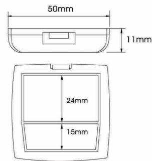
YH-E534A SIZE:W50*H11mm
