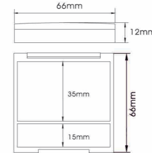
YH-E515F SIZE:W66*H12mm
