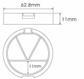
YH-E518D SIZE:W62.8*H11mm
