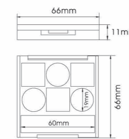
YH-E353K SIZE:W66*H11mm
