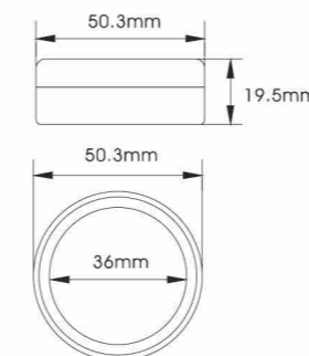
YH-E550A SIZE:W50.3*H19.5mm
