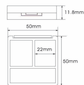
YH-E512G SIZE:W50*H11.8mm
