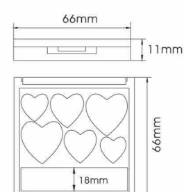
YH-E353T SIZE:W66*H11mm
