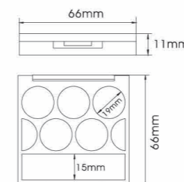
YH-E353N SIZE:W66*H11mm
