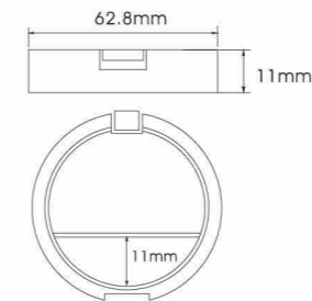
YH-E518B SIZE:W62.8*H11mm
