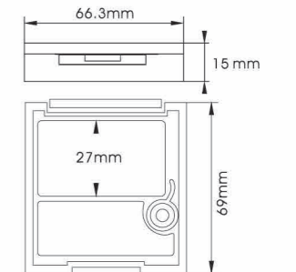
YH-E513A SIZE:L66.3*W69*H15mm
