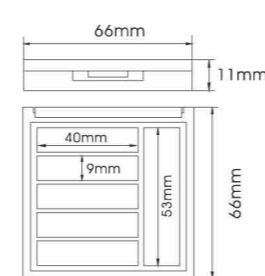
YH-E353I SIZE:W66*H11mm
