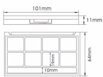
YH-E284F SIZE:L101*W64*H11mm
