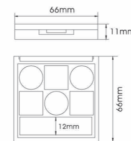
YH-E353J SIZE:W66*H11mm
