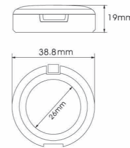
YH-E536B SIZE:W38.8*H19mm
