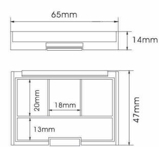
YH-E522C SIZE:L65*W47*H14mm
