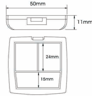
YH-E534B SIZE:W50*H11mm
