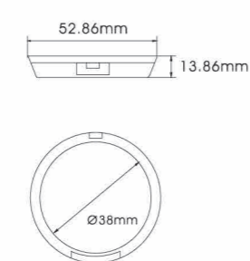
YH-E569 SIZE:W52.86*H13.86mm
