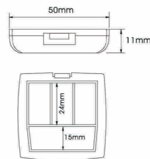
YH-E534C SIZE:W50*H11mm
