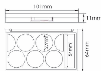
YH-E284J SIZE:L101*W64*H11mm
