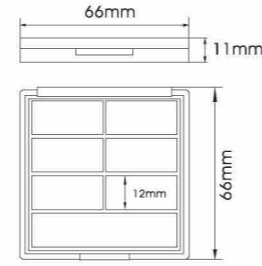
YH-E353X SIZE:W66*H11mm
