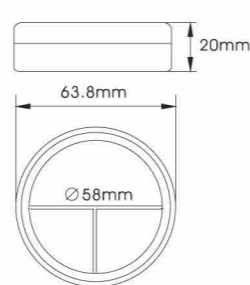
YH-E521C SIZE:W63.8*H20mm
