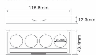
YH-E551G SIZE:L115.8*W43.4*H12.3mm
