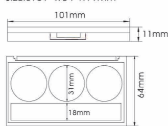
YH-E284H SIZE:L101*W64*H11mm
