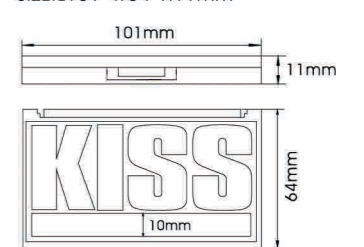
YH-E284X SIZE:L101*W64*H11mm
