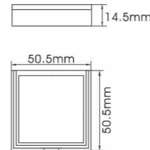
YH-E575C SIZE:L50.5*W50.5*H14.5mm
