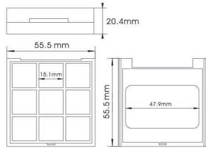
YH-E565 SIZE:L55.5*W55.5*H20.4mm
