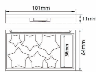
YH-E284U SIZE:L101*W64*H11mm
