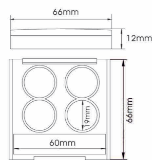
YH-E515C SIZE:W66*H12mm
