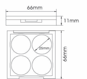
YH-E353AU SIZE:W66*H11mm
