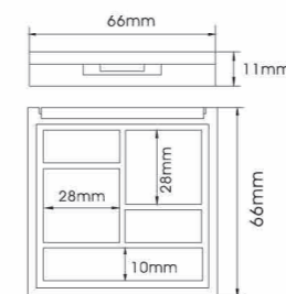
YH-E353AD SIZE:W66*H11mm
