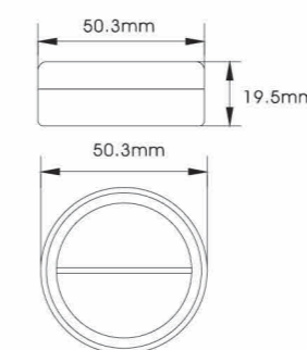
YH-E550B SIZE:W50.3*H19.5mm
