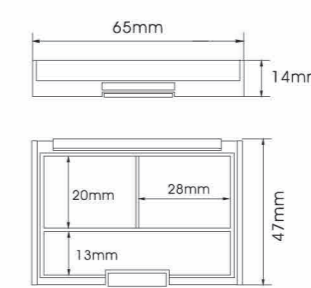
YH-E522B SIZE:L65*W47*H14mm
