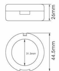
YH-E579 SIZE:W44.5*H26mm
