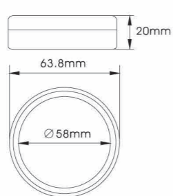
YH-E521 SIZE:W63.8*H20mm
