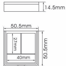
YH-E575B SIZE:L50.5*W50.5*H14.5mm
