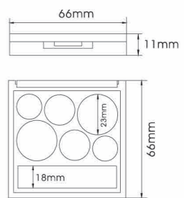
YH-E353M SIZE:W66*H11mm
