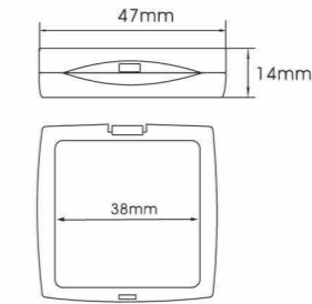
YH-E582A SIZE:W47*H14mm
