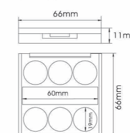
YH-E353O SIZE:W66*H11mm
