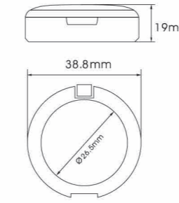
YH-E536C SIZE:W38.8*H19mm
