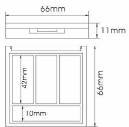
YH-E353C SIZE:W66*H11mm
