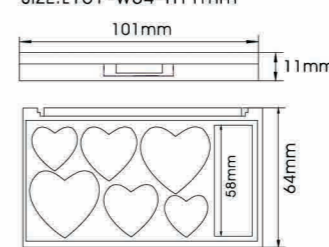
YH-E284V SIZE:L101*W64*H11mm
