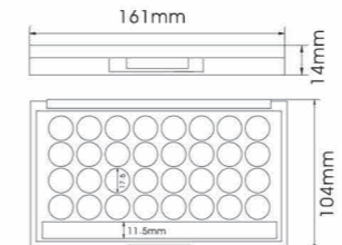
YH-E572D SIZE:L161*W104*H14mm
