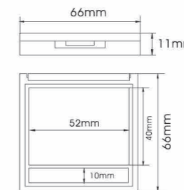
YH-E353AF SIZE:W66*H11mm
