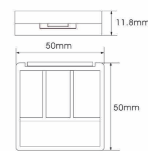
YH-E512H SIZE:W50*H11.8mm
