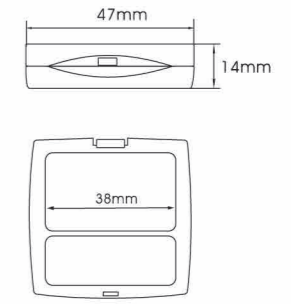
YH-E582B SIZE:W47*H14mm
