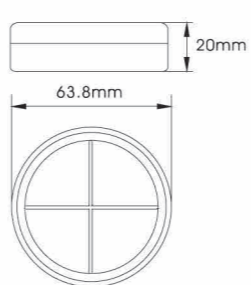
YH-E521D SIZE:W63.8*H20mm
