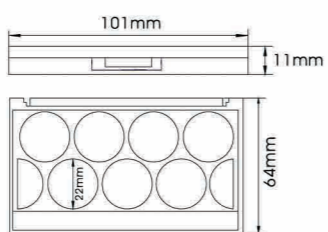
YH-E284L SIZE:L101*W64*H11mm
