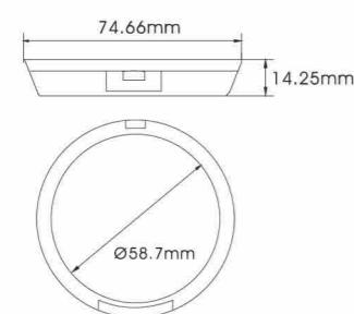
YH-E568 SIZE:W74.66*H14.25mm
