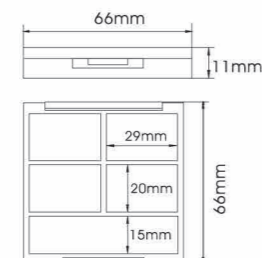
YH-E353D SIZE:W66*H11mm
