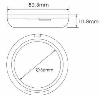
YH-E511 SIZE:W50.3*H10.8mm
