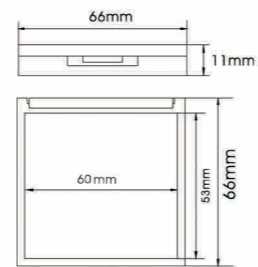
YH-E353A SIZE:W66*H11mm
