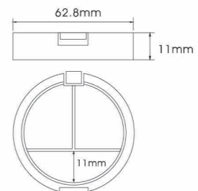
YH-E518C SIZE:W62.8*H11mm
