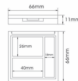
YH-E353F SIZE:W66*H11mm
