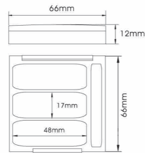
YH-E515B SIZE:W66*H12mm
