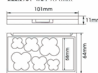
YH-E284W SIZE:L101*W64*H11mm
