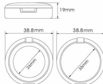
YH-E536 SIZE:W38.8*H19mm
