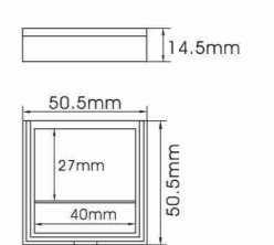
YH-E575A SIZE:L50.5*W50.5*H14.5mm
