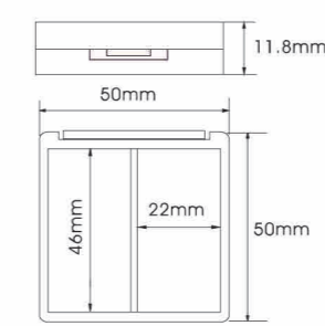
YH-E512C SIZE:W50*H11.8mm
