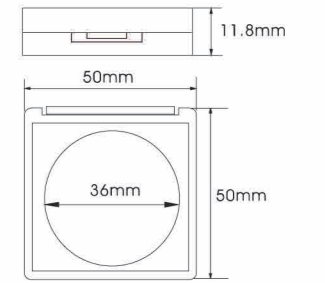
YH-E512F SIZE:W50*H11.8mm
