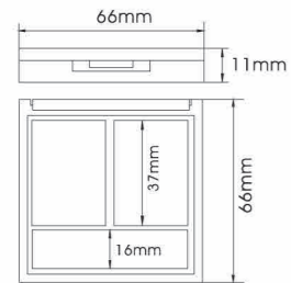
YH-E353B SIZE:W66*H11mm
