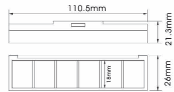
YH-E576 SIZE:L110.5*W26*H21.3mm
