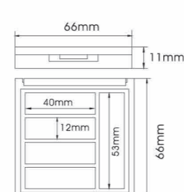
YH-E353H SIZE:W66*H11mm
