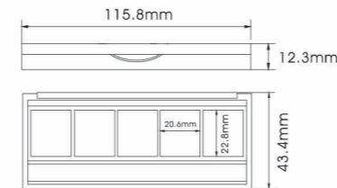
YH-E551D SIZE:L115.8*W43.4*H12.3mm
