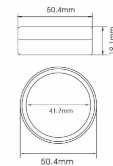
YF-E573 SIZE:W50.4*H19.1mm
