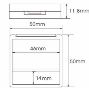
YH-E512B SIZE:W50*H11.8mm
