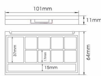
YH-E284G SIZE:L101*W64*H11mm
