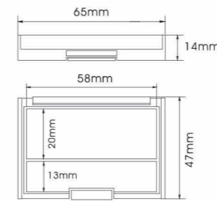
YH-E522A SIZE:L65*W47*H14mm
