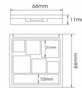
YH-E353L SIZE:W66*H11mm
