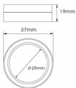
YH-E520 SIZE:W37*H19mm
