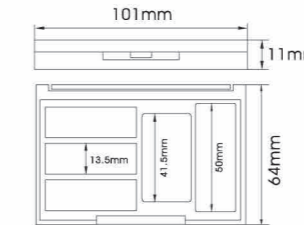
YH-E284A SIZE:L101*W64*H11mm
