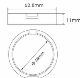
YH-E518A SIZE:W62.8*H11mm
