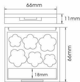
YH-E353U SIZE:W66*H11mm
