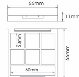
YH-E353E SIZE:W66*H11mm
