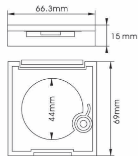
YH-E513B SIZE:L66.3*W69*H15mm
