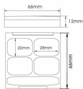
YH-E515D SIZE:W66*H12mm
