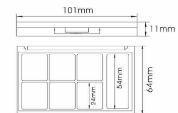
YH-E284C SIZE:L101*W64*H11mm
