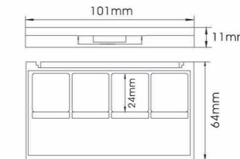
YH-E284B SIZE:L101*W64*H11mm
