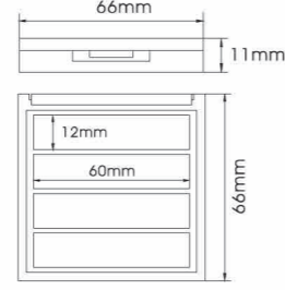
YH-E353W SIZE:W66*H11mm
