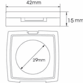
YH-E523 SIZE:W42*H15mm
