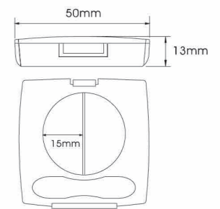
YH-E539B SIZE:W50*H13mm
